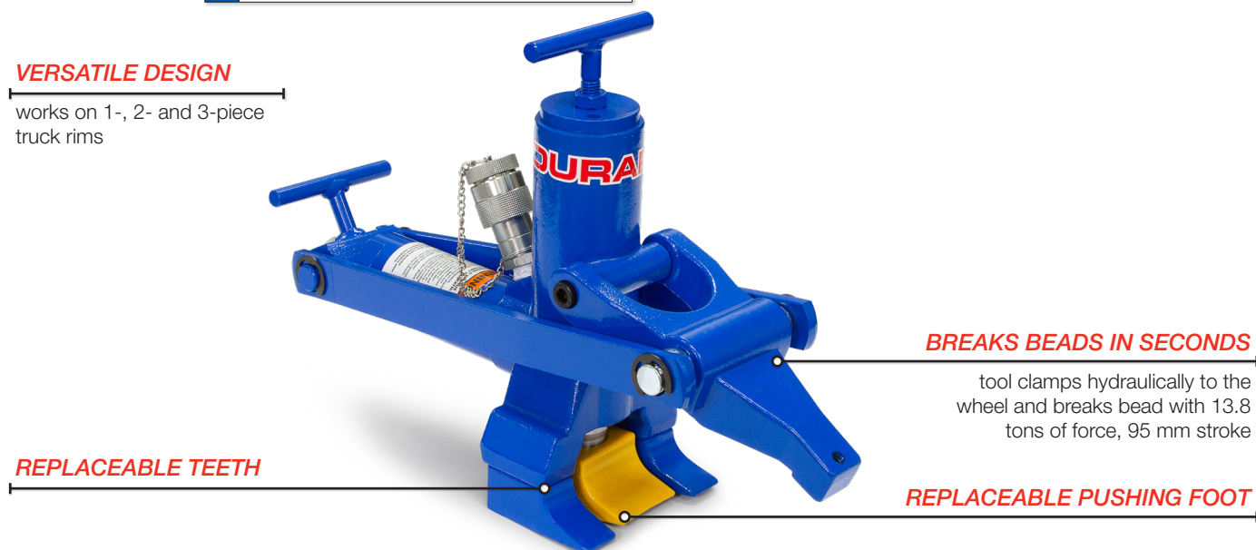
BB-6120 – Combi Tyre Bead Breaker
