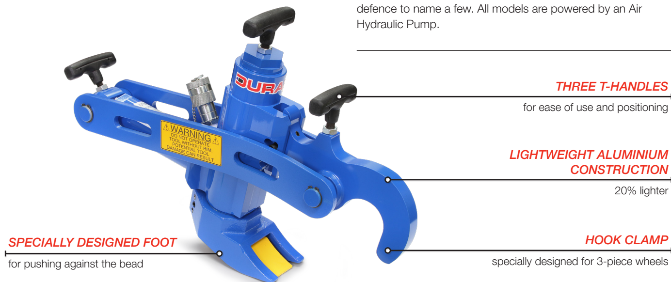
BB-6110 – Aluminium Tyre Bead Breaker
